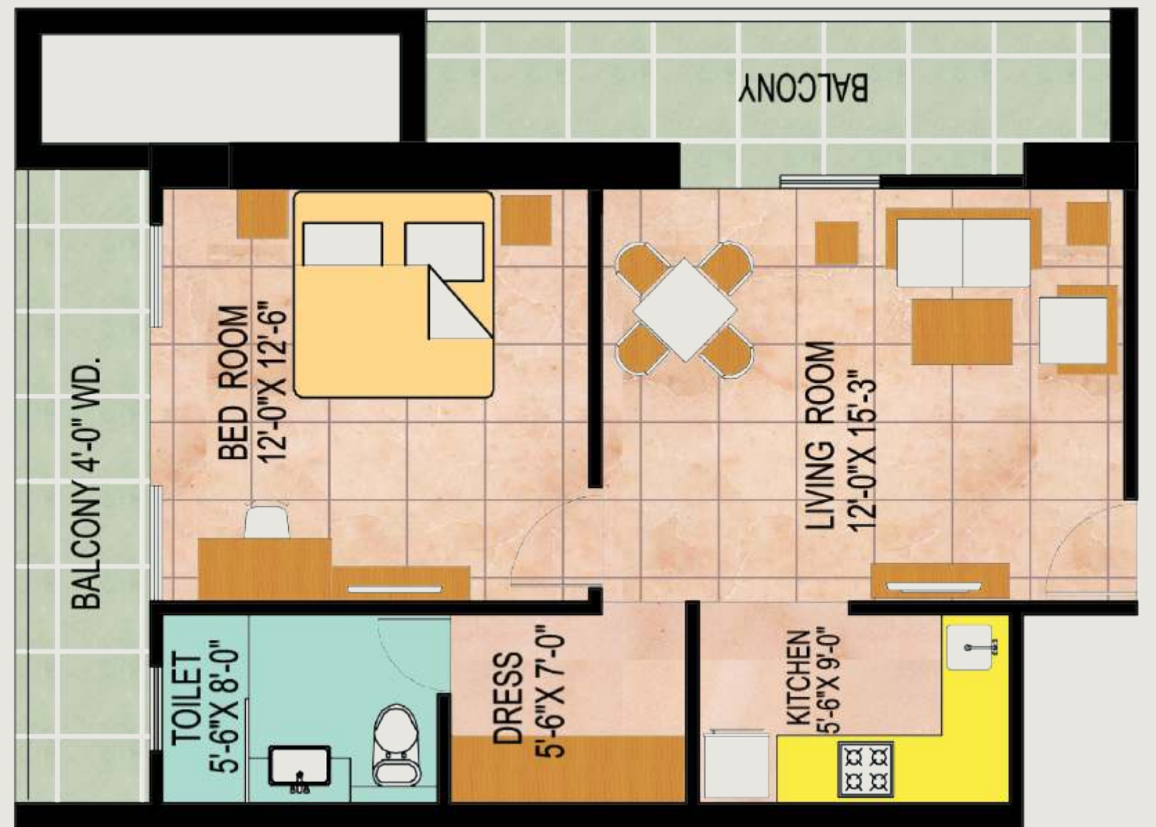
TYPE C 9TH TO 12TH FLOOR
